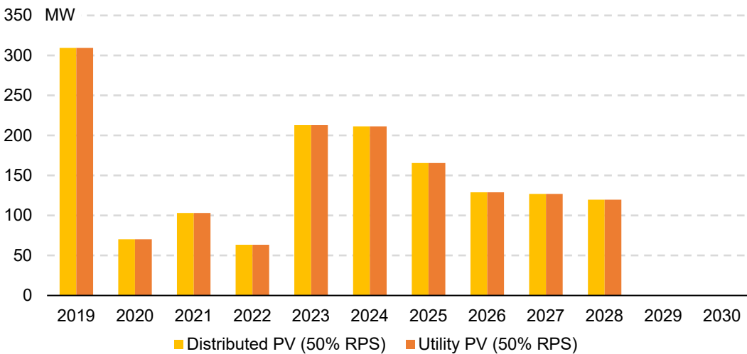
Figure 3-39. Projected Annual Solar PV Capacity Additions, 50% RPS
