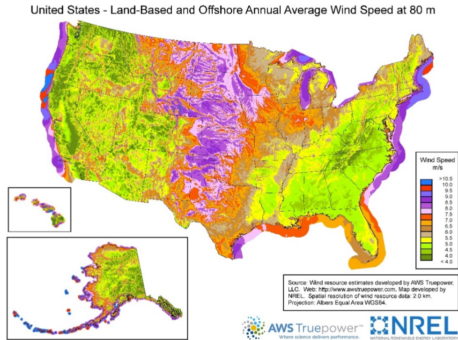
Figure 3-10. Onshore and Offshore Wind Quality in the U.S. Source: NREL, 2012, nrel.gov/gis/images/80m_wind/awstwsd80onoffbigC3-3dpi600.jpg .
