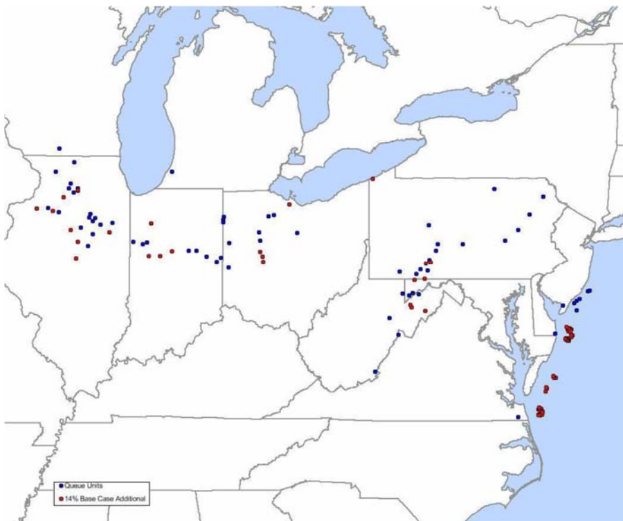
Figure J-1. Wind Sites, PRIS 14% Base Case
