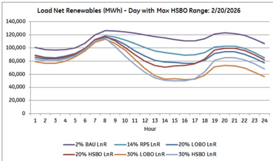
Figure J-5. Hourly Net Load Profile Under Different PRIS Scenarios
