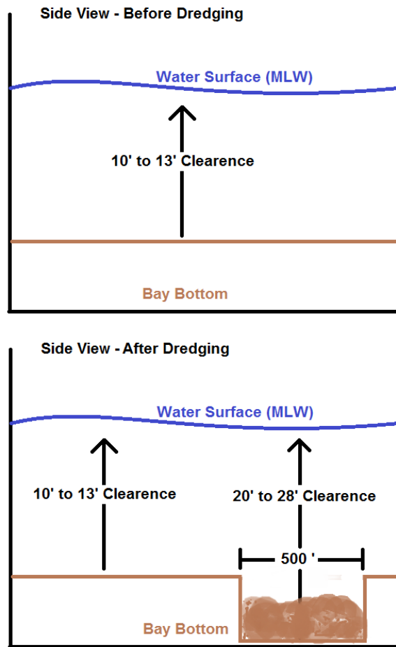
Figure 2. A stylized cross section of the proposed dredge cuts to be made at Man-O-War shoal. Actual cut sides and bottoms are not at precise right angles.
