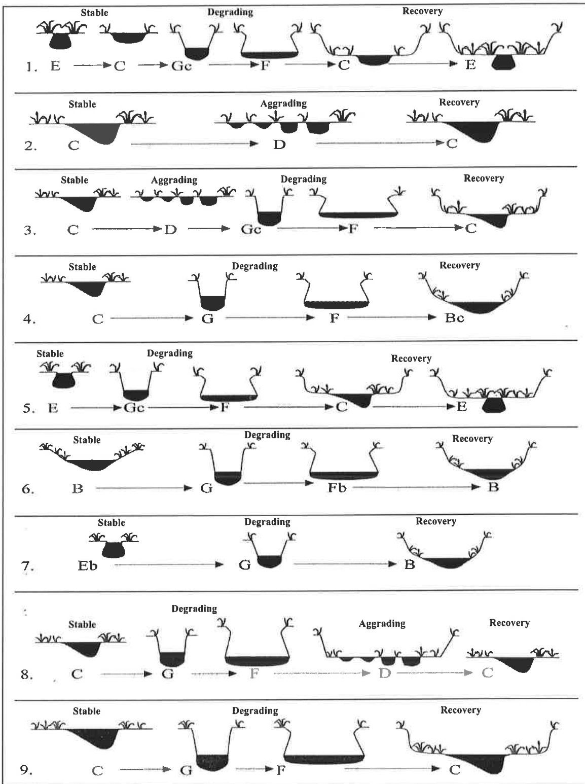
Figure 8. Various Stream Type Succession Scenarios (Rosgen 2001b)
