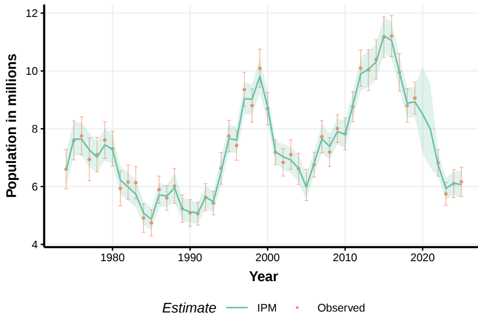
Figure 3 – Population estimates of mid-continent mallards observed from the WBPHS compared to mid-continent mallard integrated population model (IPM) predictions from 1974–2025. Error bars represent 95% confidence intervals while the error bands (line shading) represent 95% credibility intervals.
