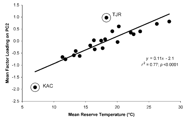
Figure 2. Relationship between mean reserve temperature and mean factor loadings on PC2.
