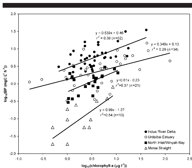
Figure 4. Estuarine systems exhibiting relatively strong covariation of BP and CHLA. All regressions are highly significant ( i.e. , p < 0.0001 ).
