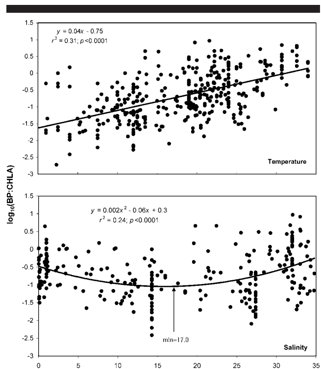
Figure 5. Relationship between log-transformed BP:CHLA ratios and (A) temperature and (B) salinity as independent variables.
