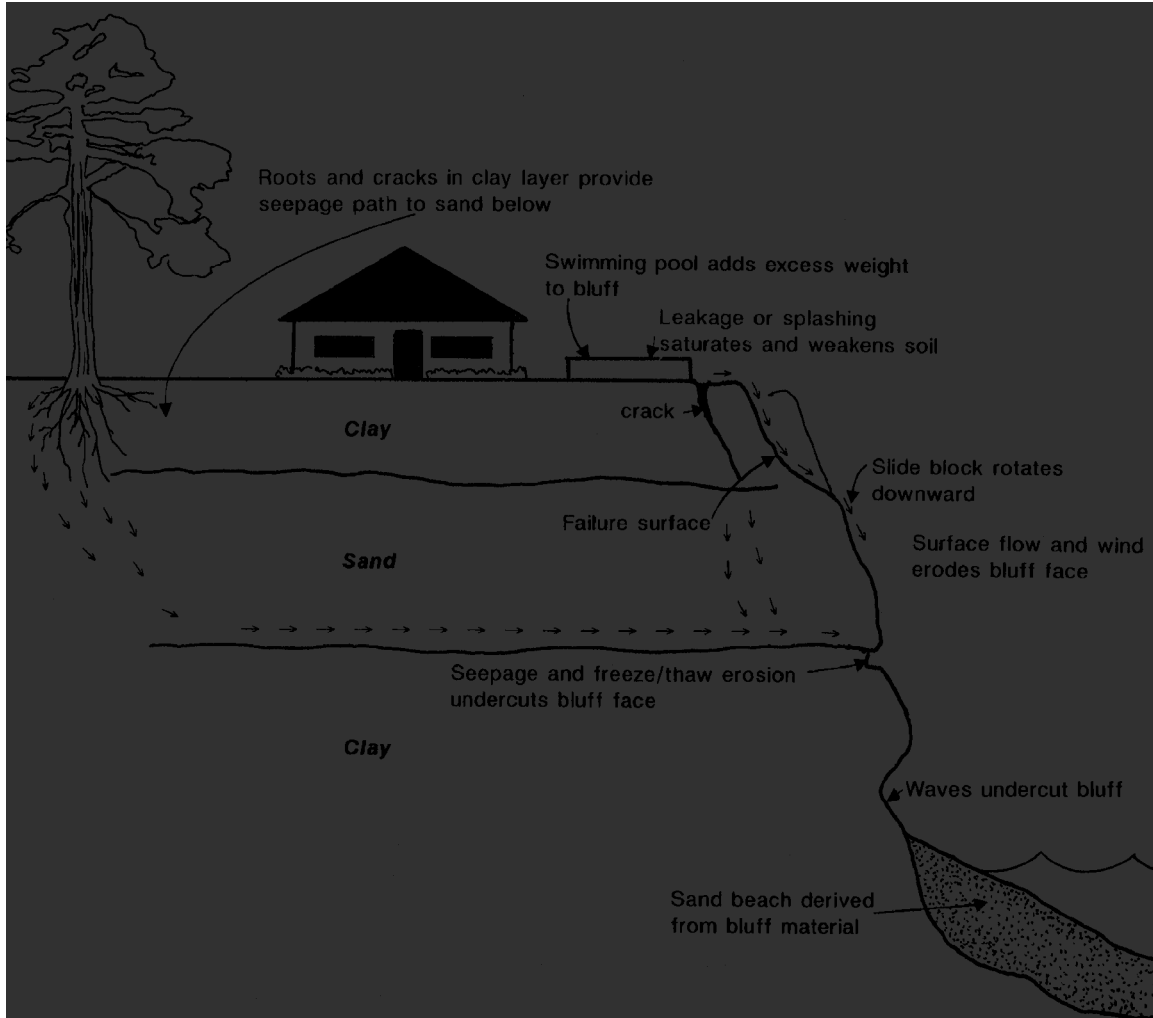
Figure 4. The combination of wave and groundwater erosion on a high bank. (DNR, 1992)
