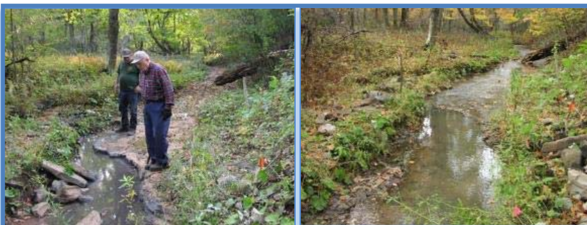
Photos During and Shortly After 2007 CCB-Grout Injection at Hoyes Run. Stream flow was restored within hours of grout injection.
