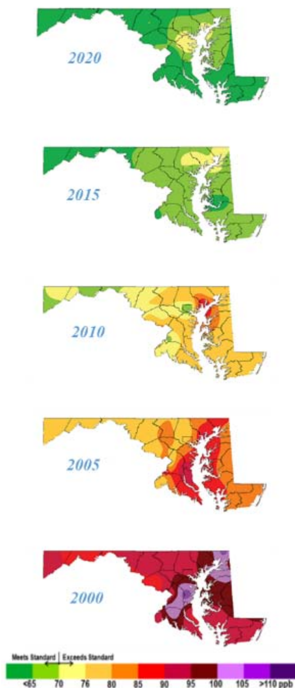
Figure 5-12 Maryland's Ozone Trend – 2000-2020
