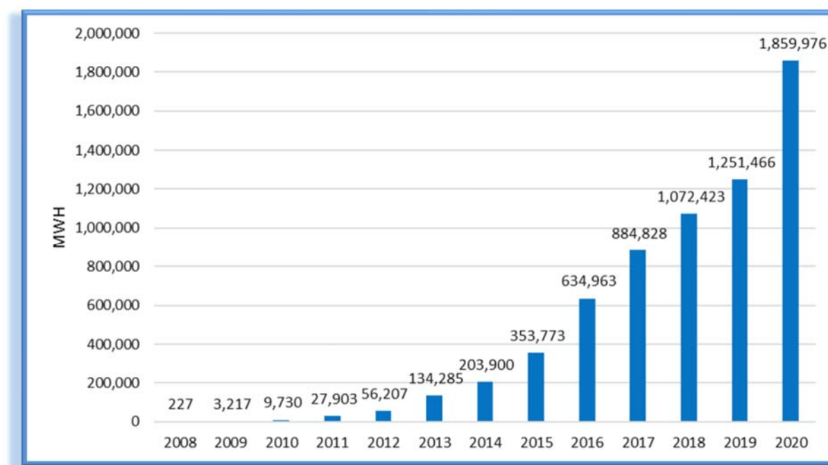
Figure 3-11 Solar Generation in Maryland, 2008-2020
