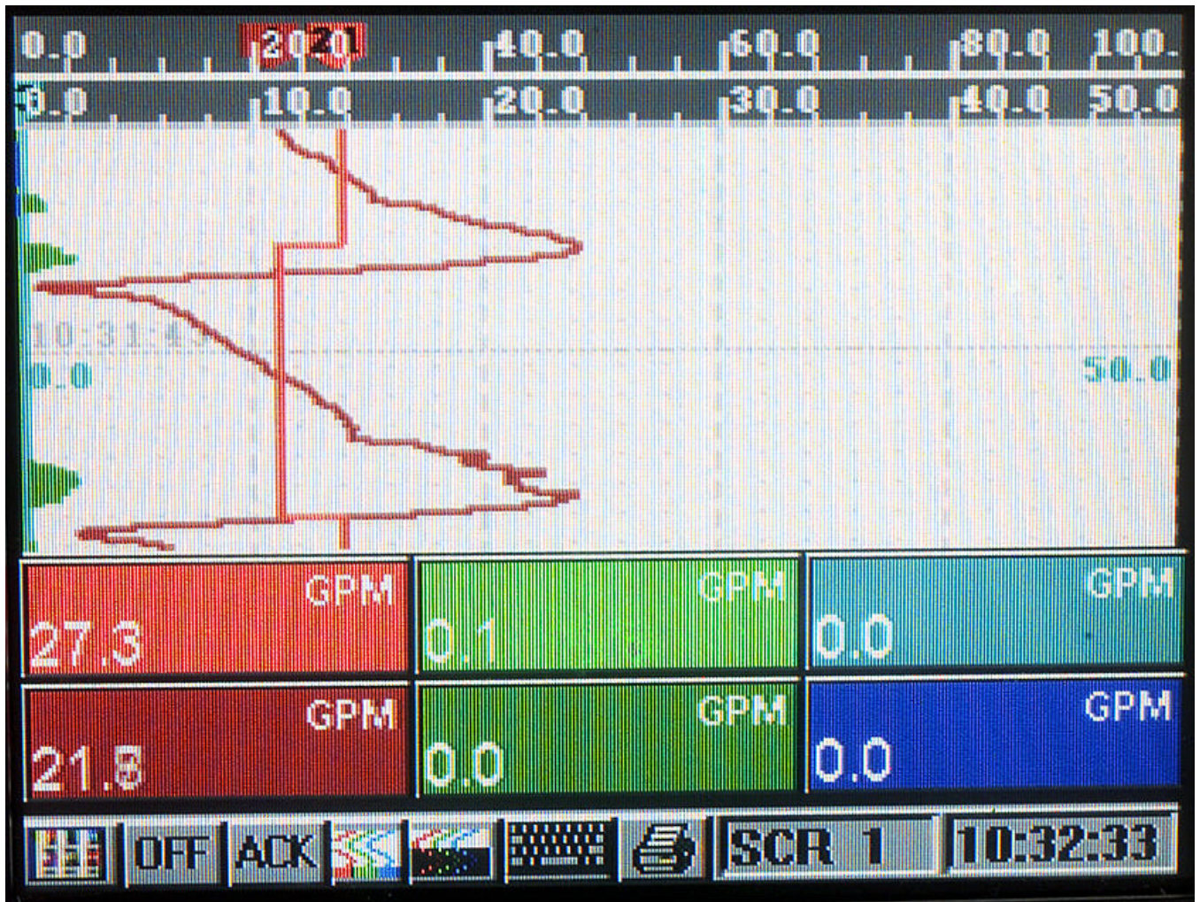
Figure 6.9 – Keco Model 1000V-3 HP Vacuum Pump-out Unit
